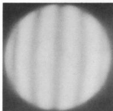
Unretouched Photos of Cave Astrola 8" F/6.7 Mirror
