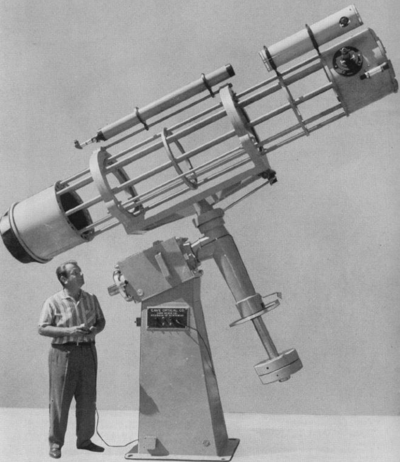
OBSERVATORY 18"
