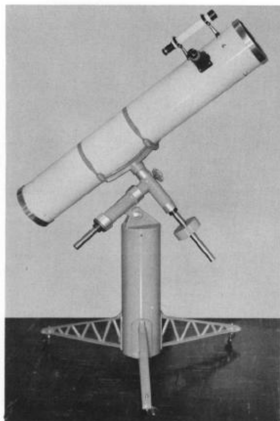
6" F/8 STUDENT STANDARD
